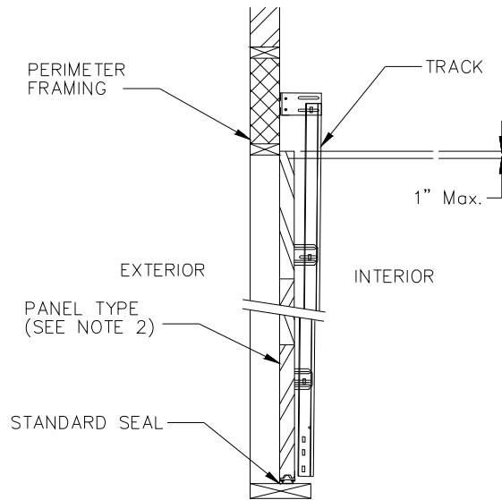
VERTICAL SECTION
