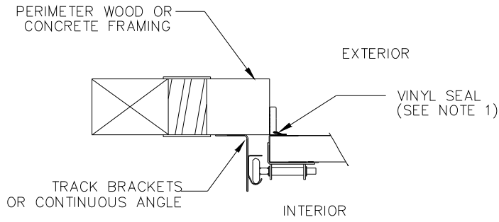
HORIZONTAL SECTION - Using Vinyl Seal
