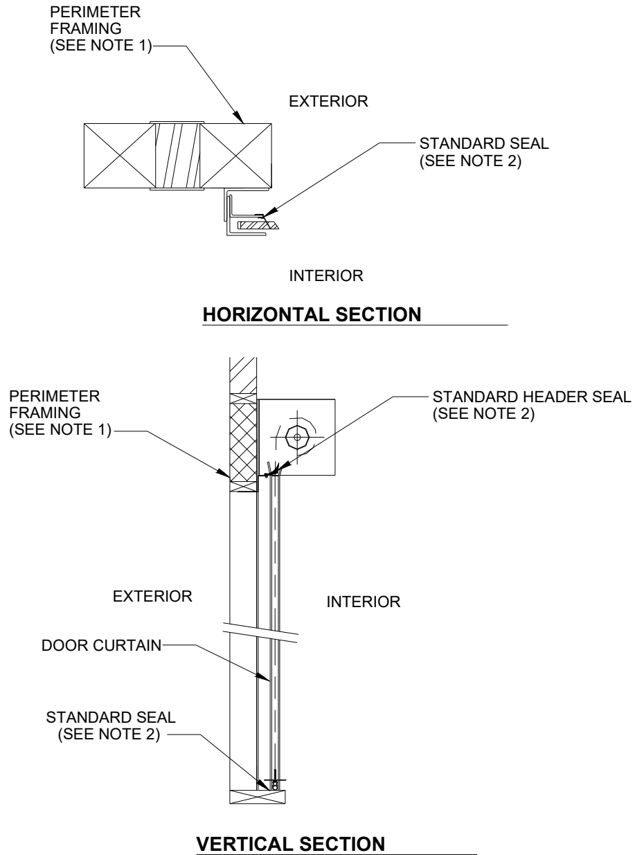
FIGURE 3A – ROLLING DOOR INSTALLATION AIR INFILTRATION TEST
