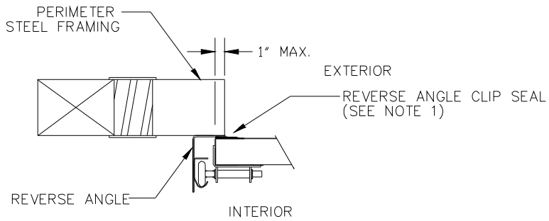
HORIZONTAL SECTION - Using Reverse Angle Clip Seal
