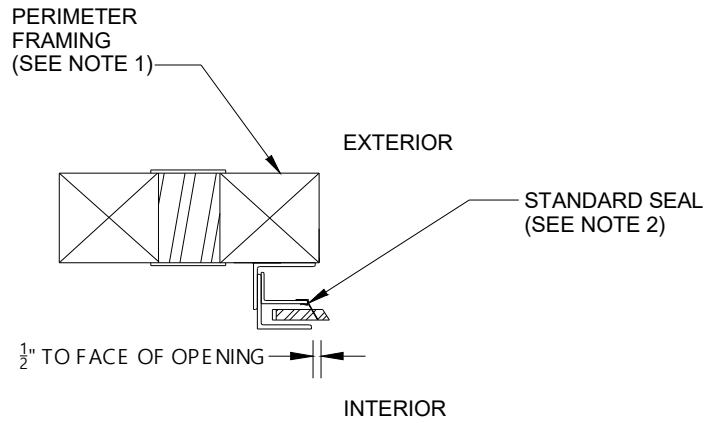
FIGURE 3 – ROLLING DOOR INSTALLATION THERMAL TRANSMITTANCE TEST
