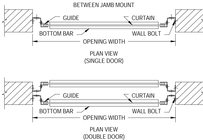
Figure 3 Rolling Steel Doors – Between-Jamb Mounted (source: NFPA 80)
