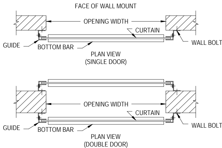
Figure 2 Rolling Steel Doors – Face Mounted (source: NFPA 80)
